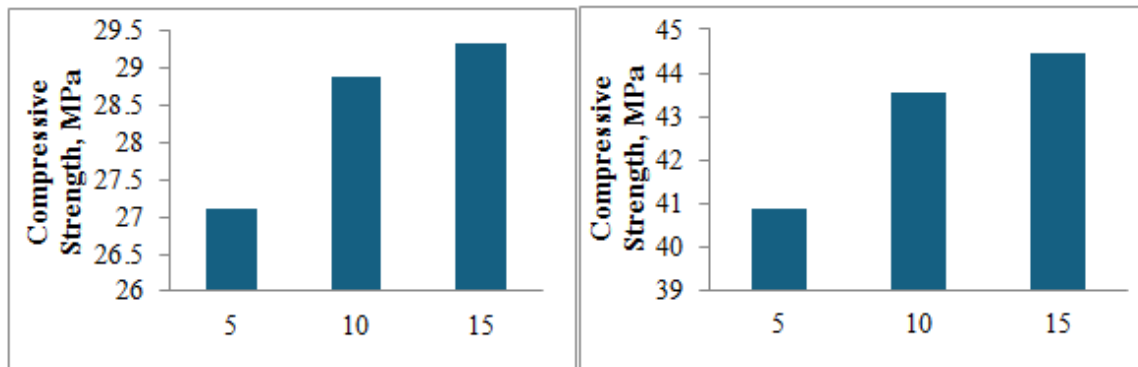
(a) Compressive strength at 7 days (b) Compressive strength at 28 days
