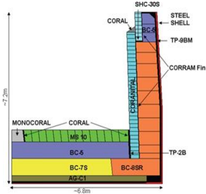
Figure 6: Design of BF4 at Dillinger Hüttenwerke
