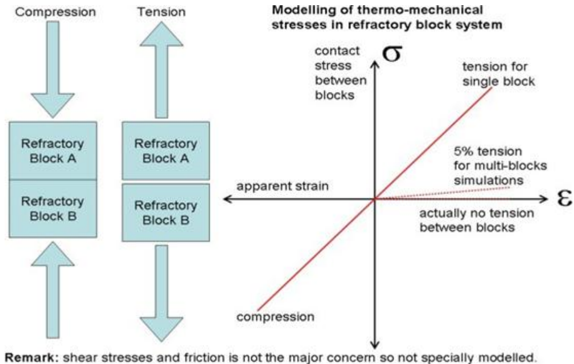
Figure 1: No Tension Concept
