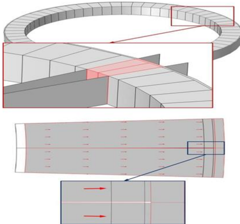
Figure 2: Separation and contact of block
