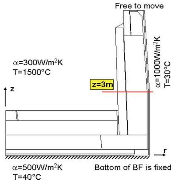
Figure 7: Simulated geometry and BCs
