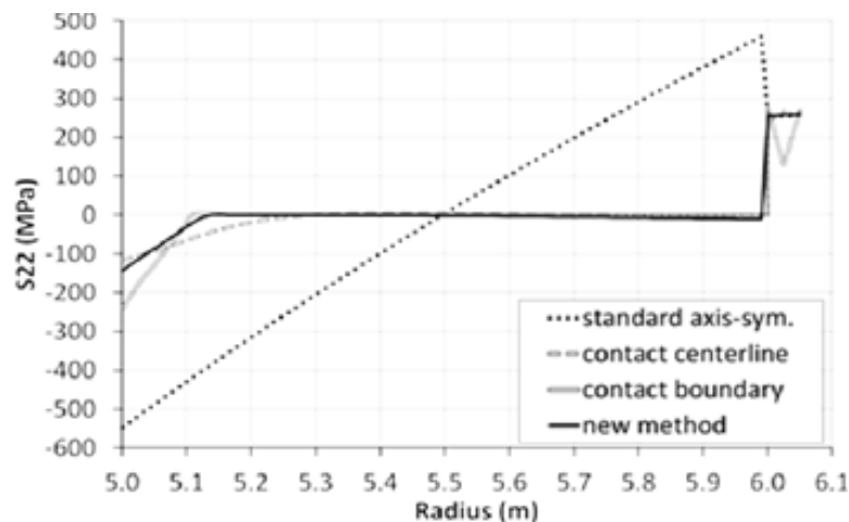
Figure 5: Comparison of hoop stresses The radial displacements of the steel shell are:
