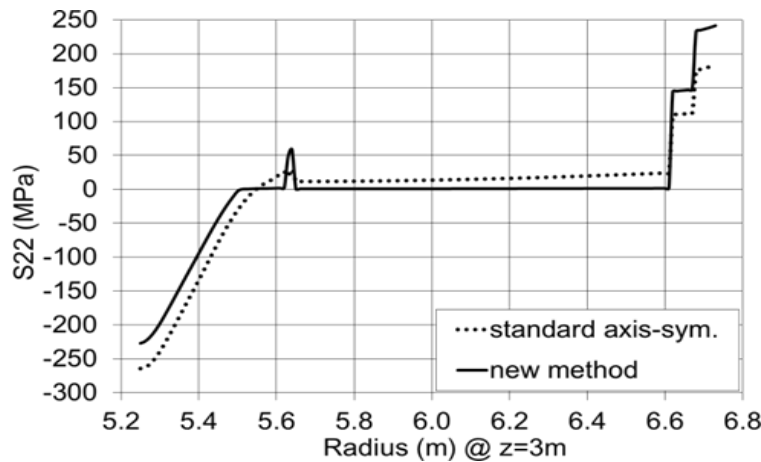
Figure 8: Hoop stress ( \sigma_{\phi\phi} ) at the cut line ( z=3m )
