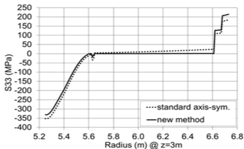
Figure 9: Vertical stress ( \sigma_{zz} ) at the cut line ( z=3m )
