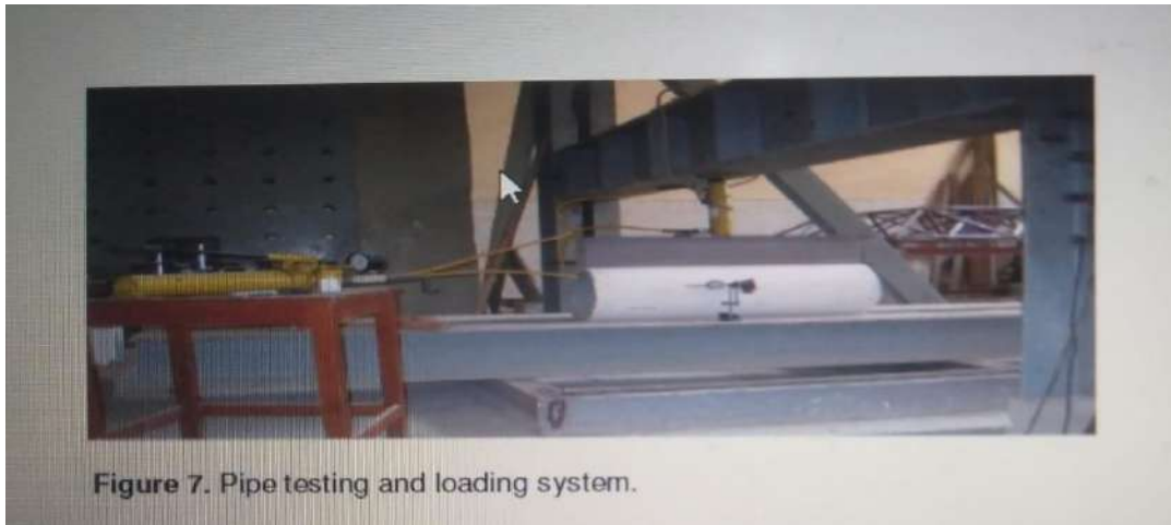
Figure 7. Pipe testing and loading system
