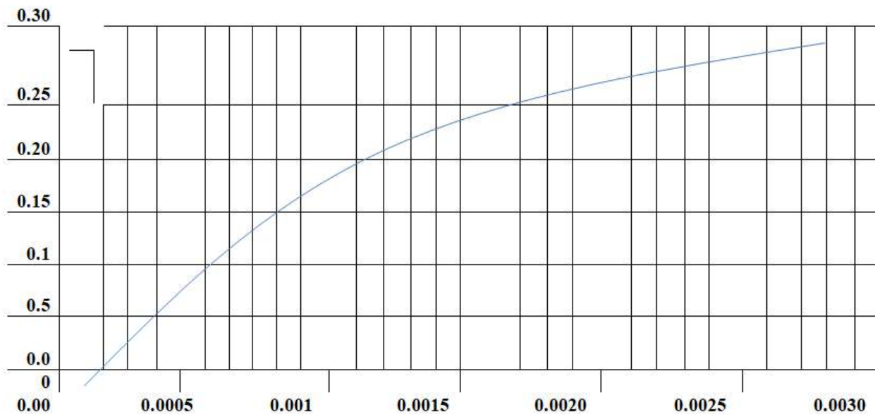
Figure 4. Stress-strain curve of the used concrete.
