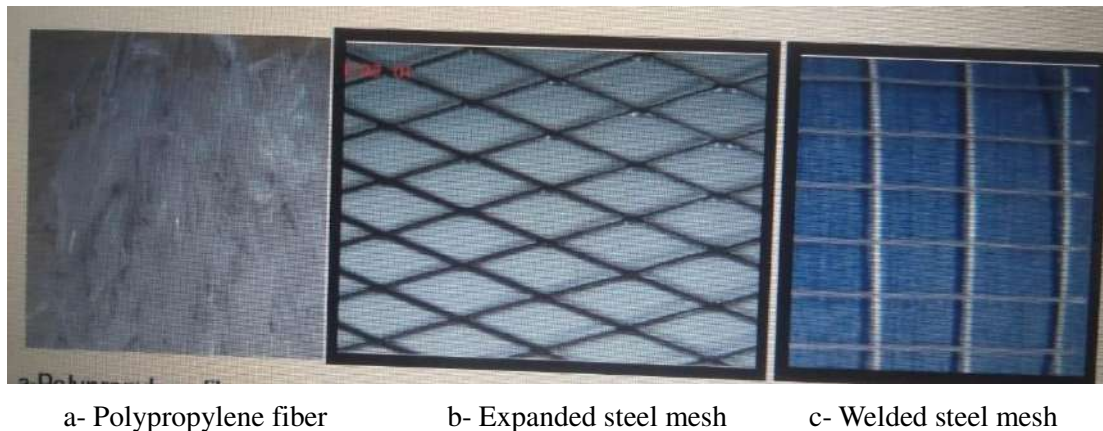
Figure 1. Reinforcement steel meshes and fibers used.
