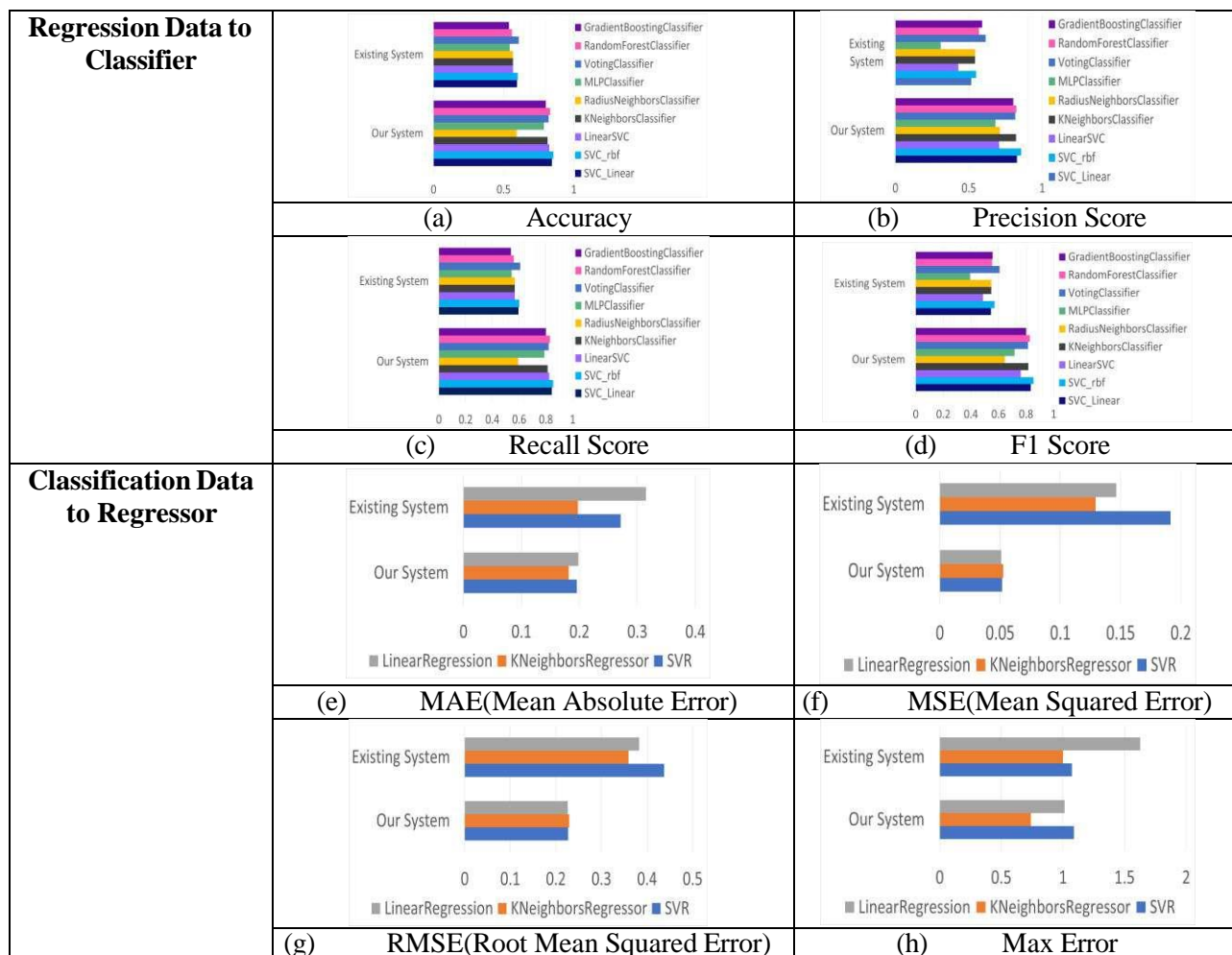
Fig 3: Regression and classification cross automatic transformation experiment results
