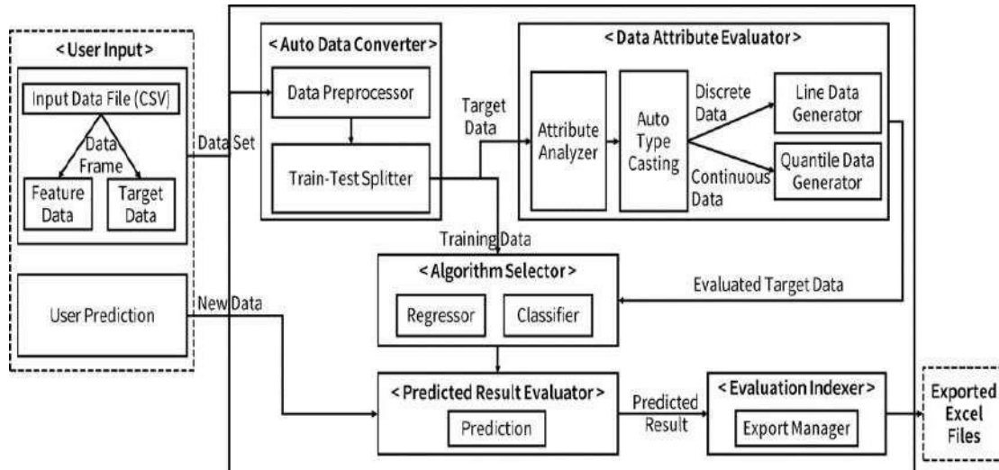
Fig 1: Proposed System Diagram
