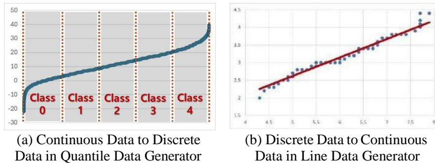
Fig 2: Data Attribute Transformation
