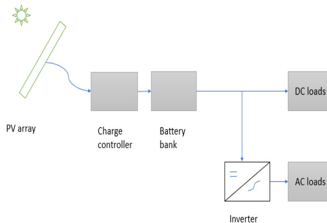
Fig.3 PV system is stand-alone (off grid)
