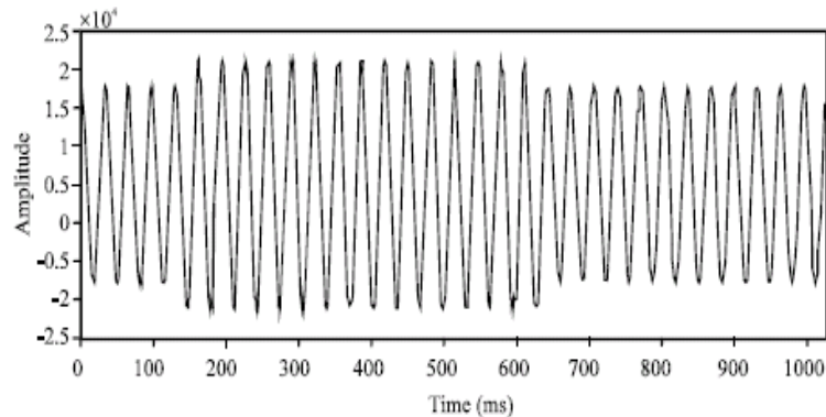
Figure 7: Voltage Swell waveform
