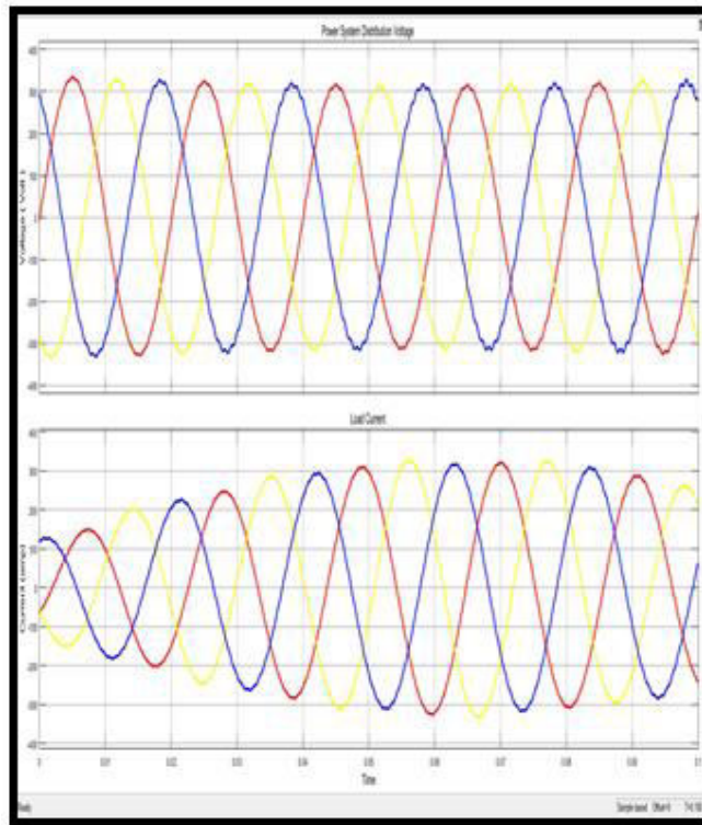
Fig 11- Grid Supply side voltage and current
