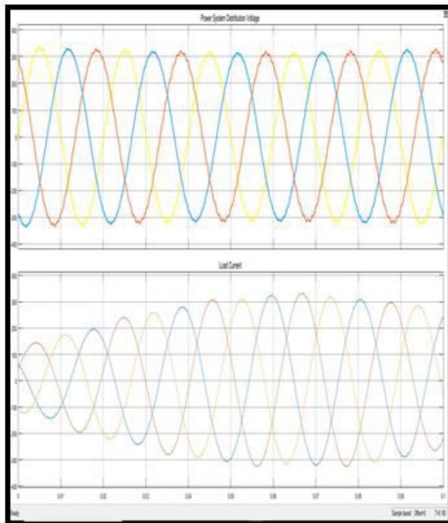
Fig 10: Distribution side hybrid output Voltage and Current
